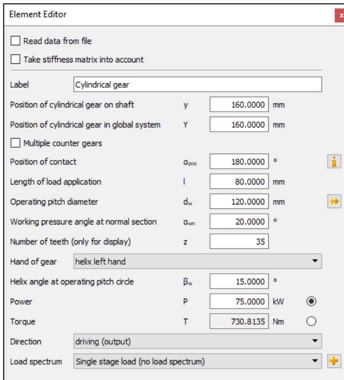
Figure 9. Definition of a machine element, using the example of a cylindrical gear
